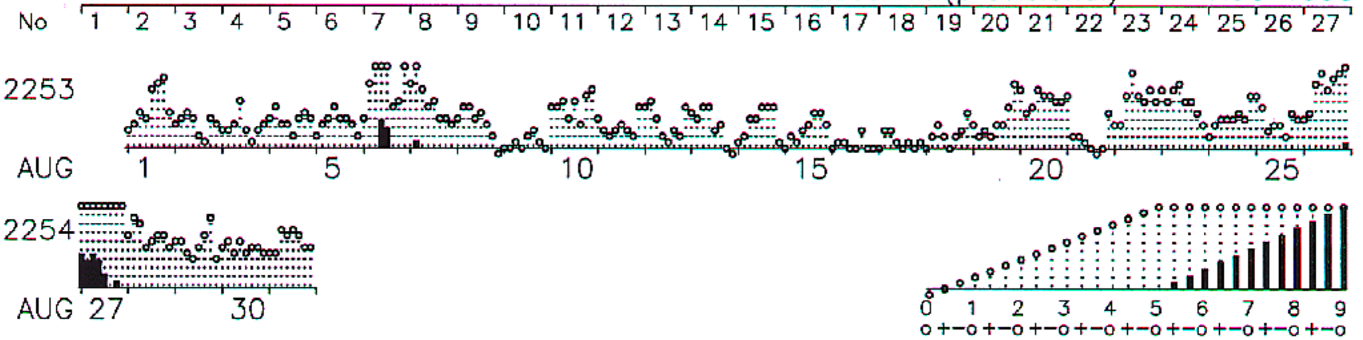
ROT DAY IN SOLAR ROTATION INTERVAL Three-hour indices aa (logscale) AUG-OCT 1998
