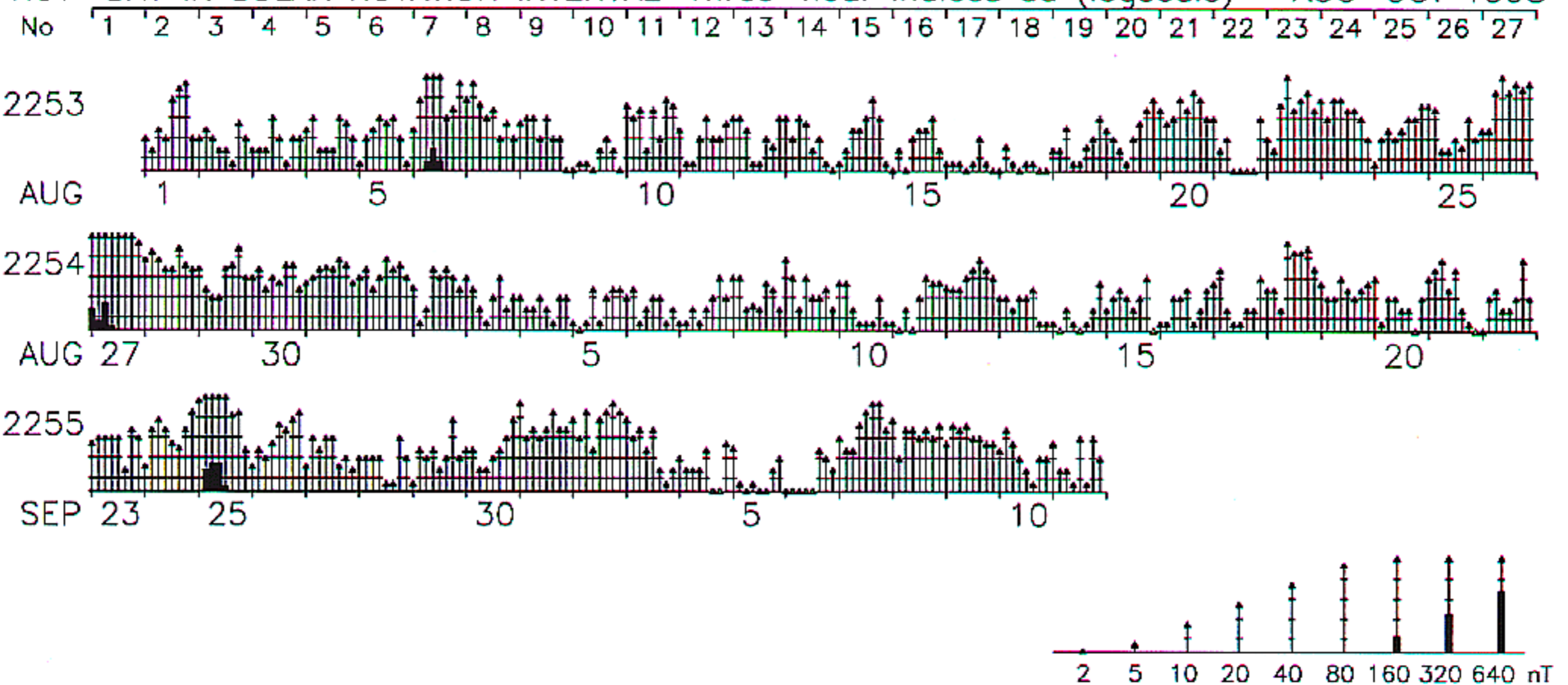
ROT DAY IN SOLAR ROTATION INTERVAL Three-hour indices aa (logscale) AUG-OCT 1998
